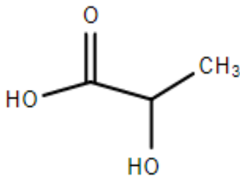
Figure 1. Lactic acid, an alpha hydroxy acid.
