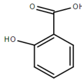
Figure 2. Salicylic acid, a beta hydroxy acid.
