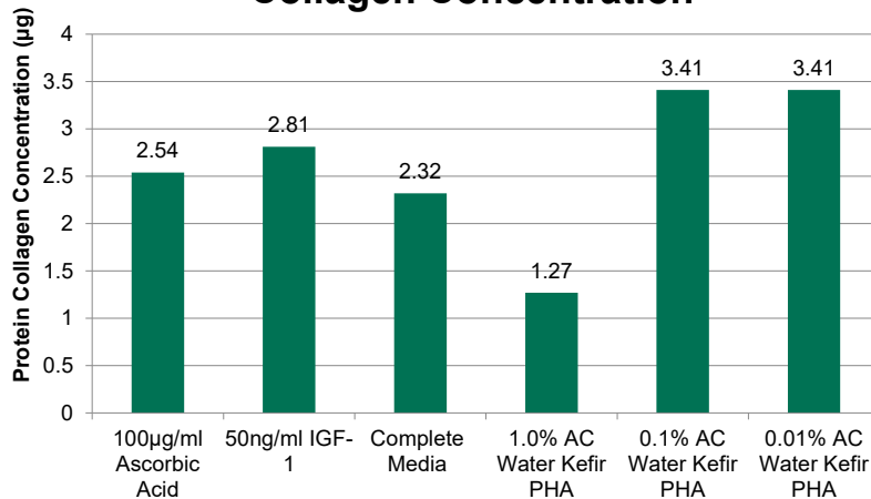
Figure 6. Collagen Concentration.
